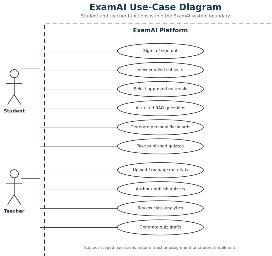
Figure 8.3: Use-case diagram
